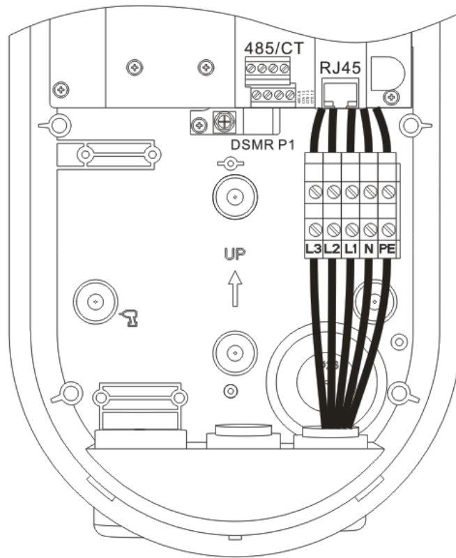
Figure 2-6 Wiring
