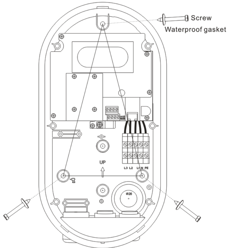
Figure 2-5 Fix the device
