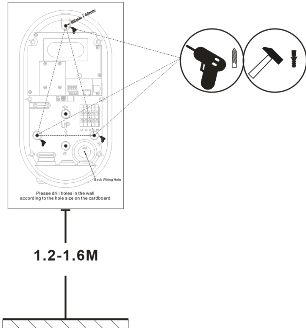
Figure 2-3 Locate the installation location
